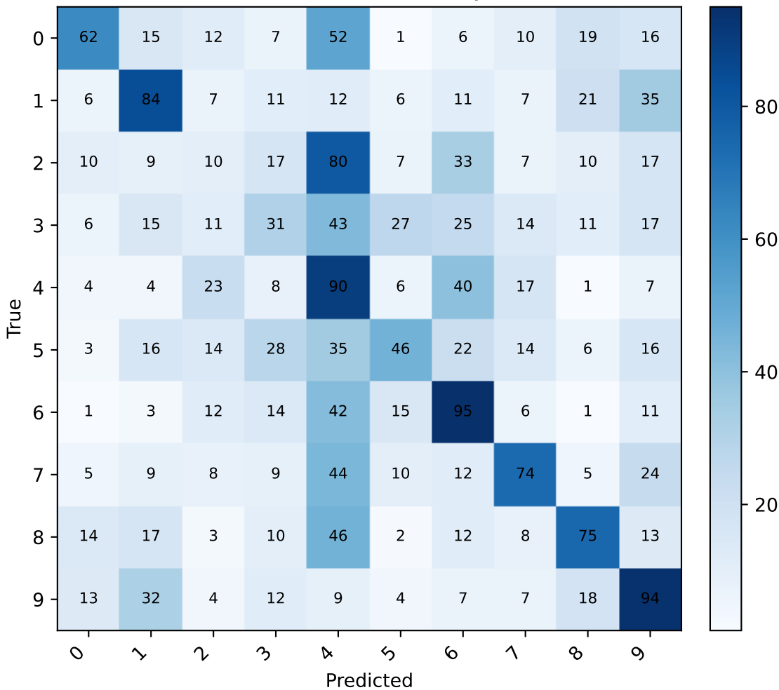
CIFAR-10 Gaussian Bayes
