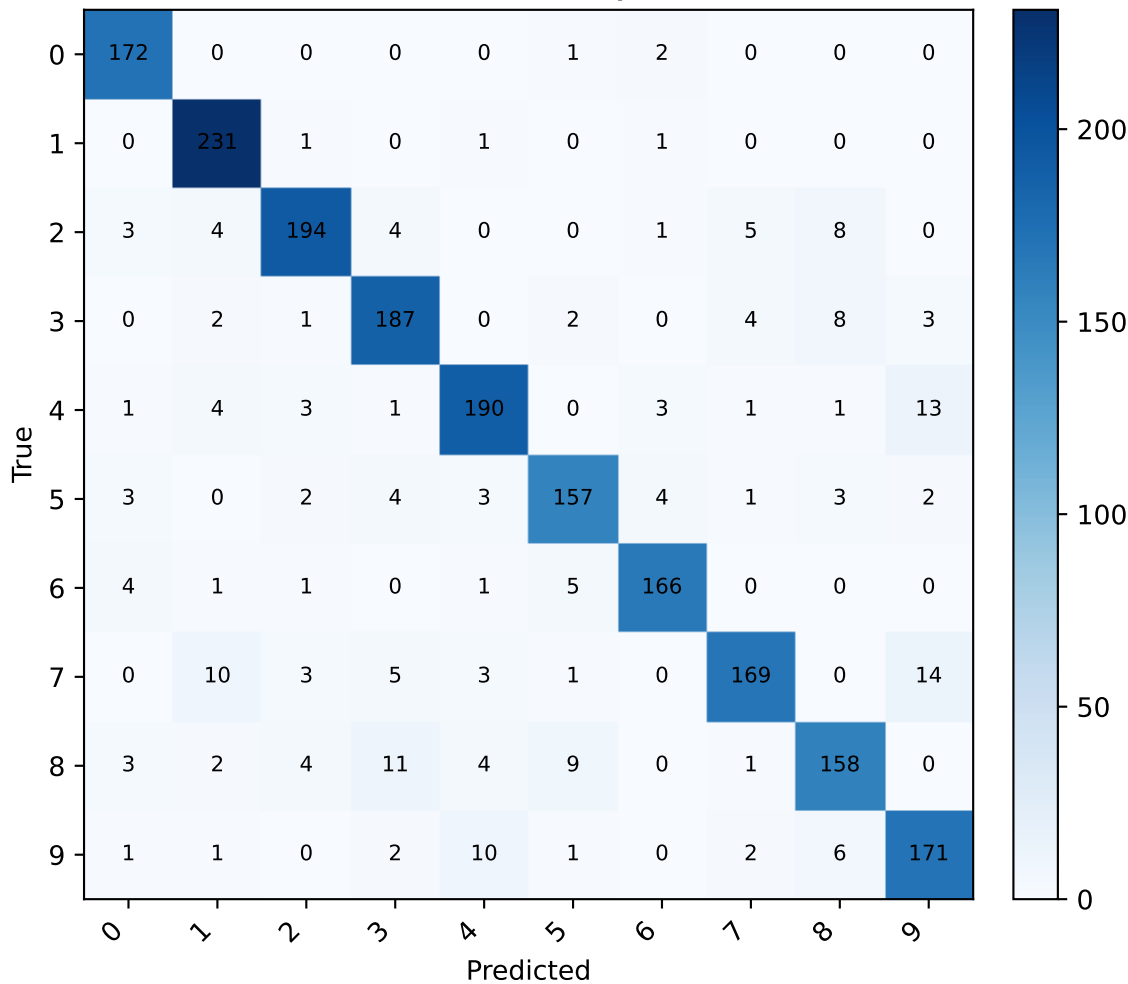
MNIST kNN Bayes
