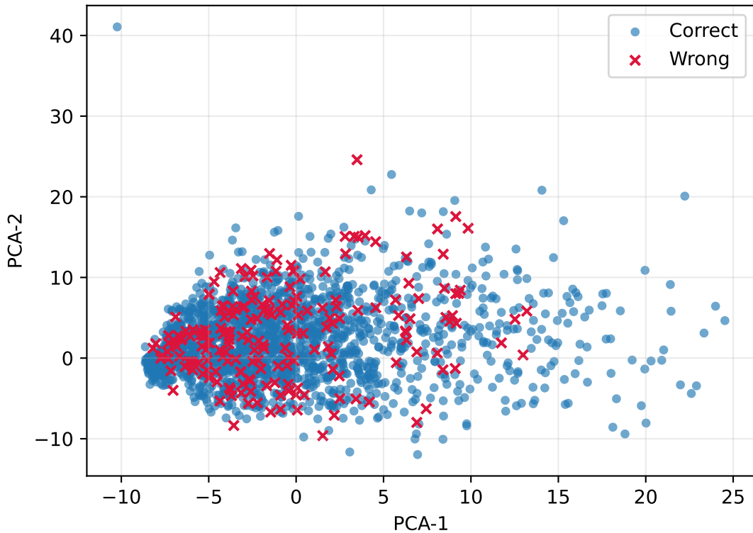
MNIST kNN prediction on PCA features
