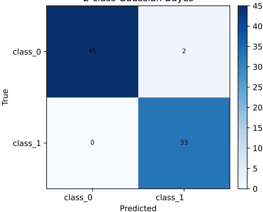
2-class Gaussian Bayes
