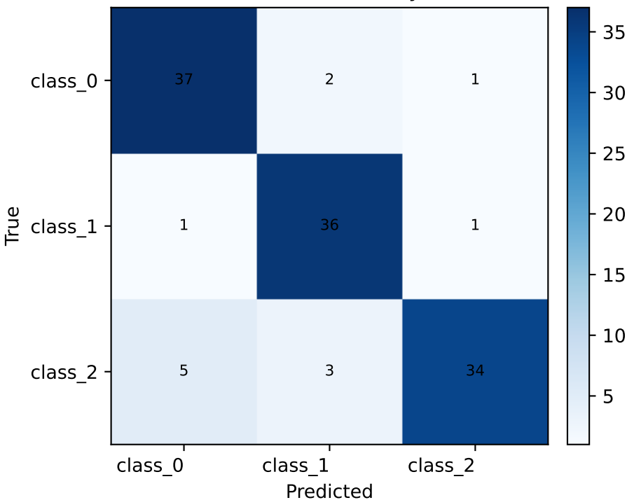
3-class Parzen Bayes
