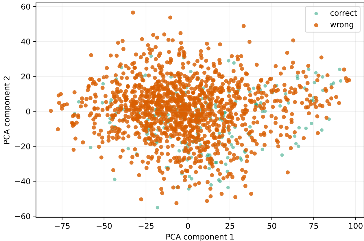
CIFAR-100 LDA prediction on PCA features
