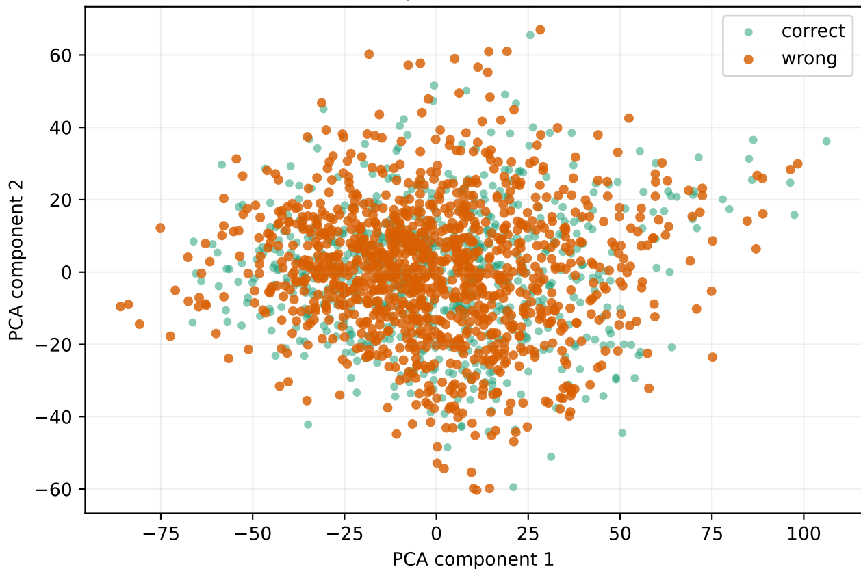
CIFAR-10 LDA prediction on PCA features
