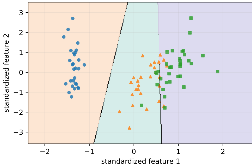
Fisher/LDA
