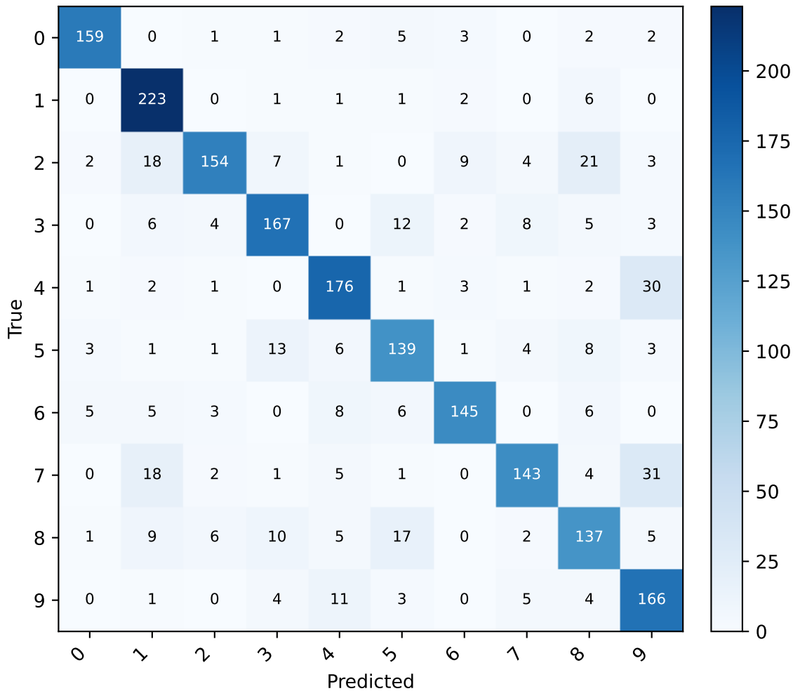
MNIST LDA
