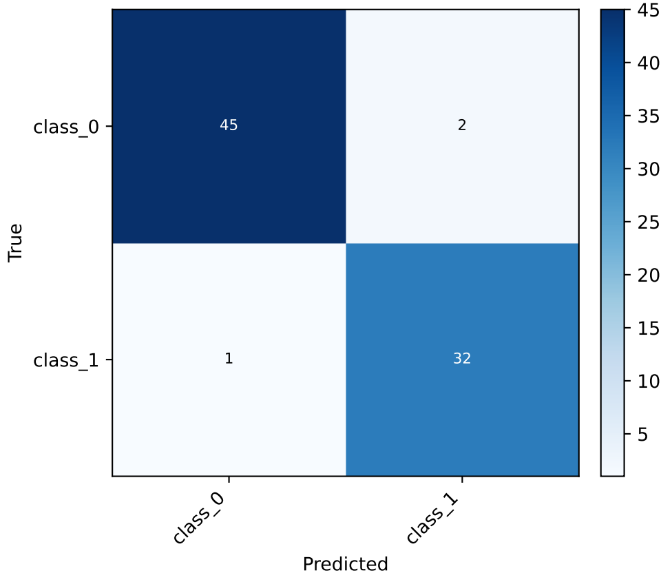
Simulated 2-class LDA
