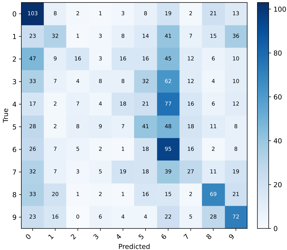
CIFAR-10 PCA+NearestCentroid
