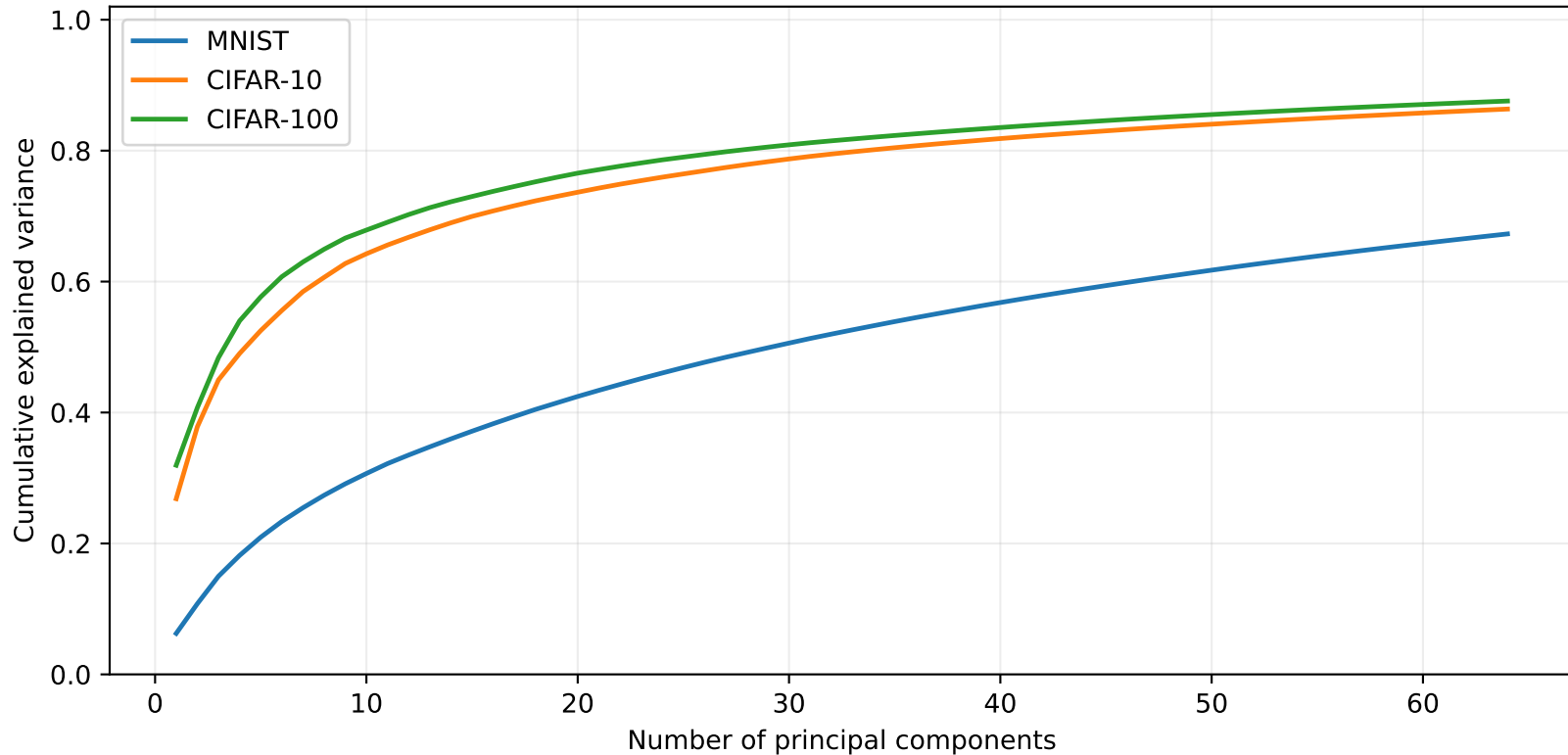
K-L/PCA Cumulative Explained Variance
