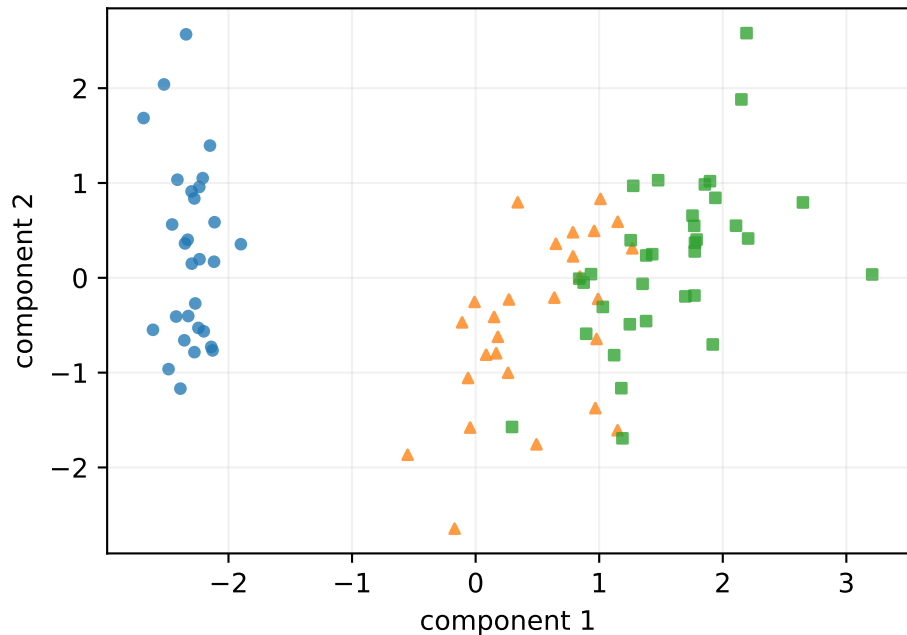
PCA/K-L projection
