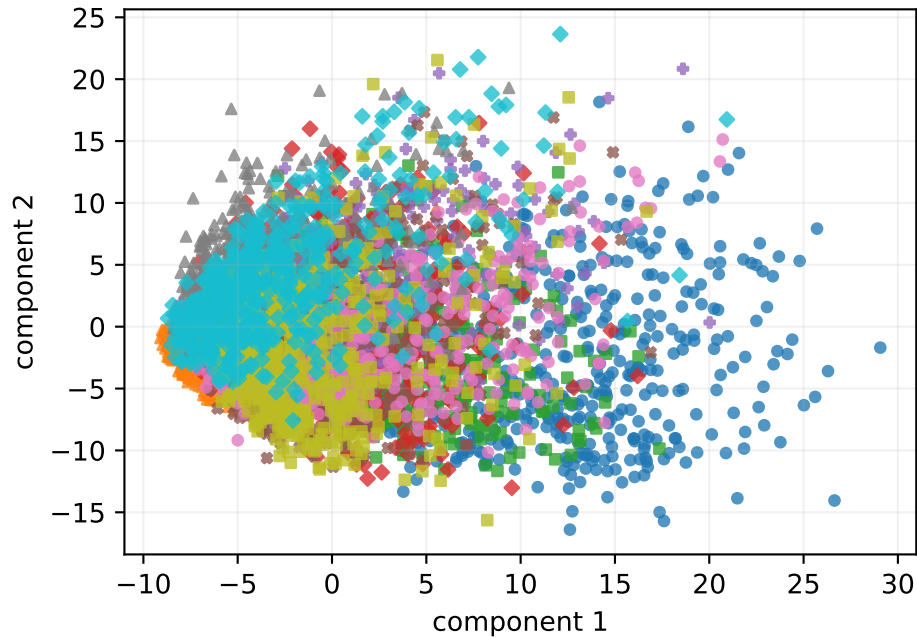
PCA/K-L projection
