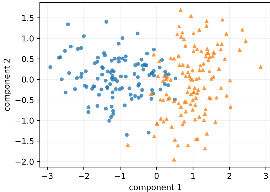
PCA/K-L projection
