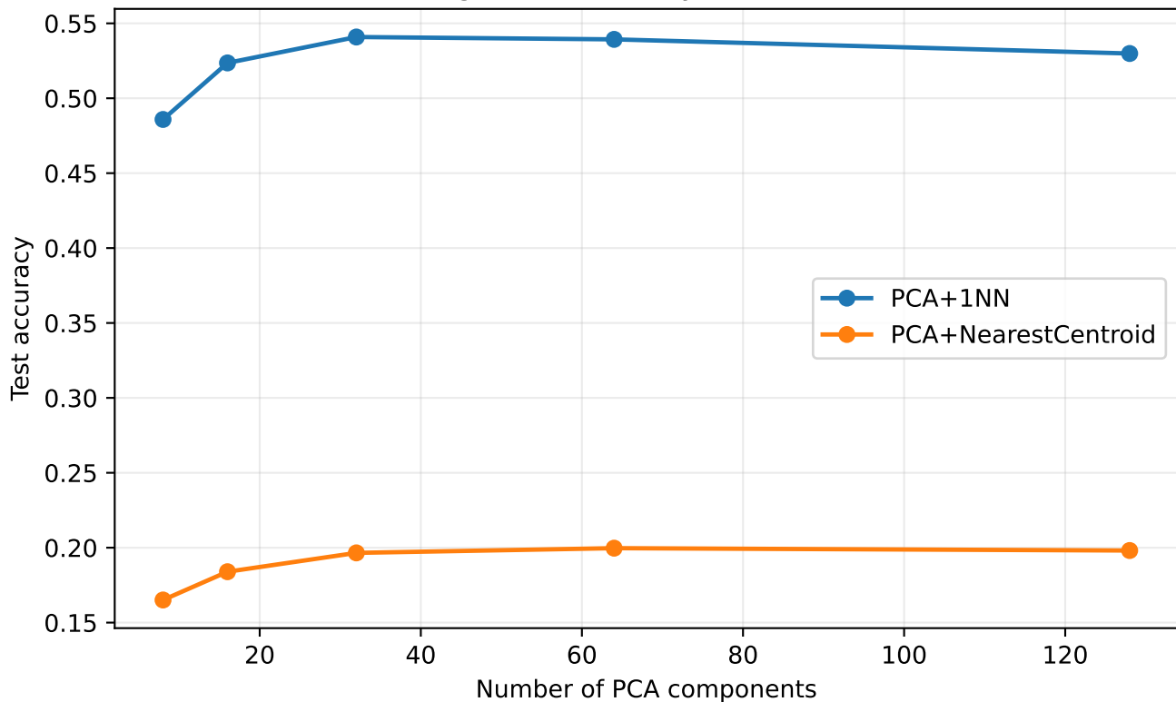
Aircraft Recognition Accuracy with K-L/PCA Features
