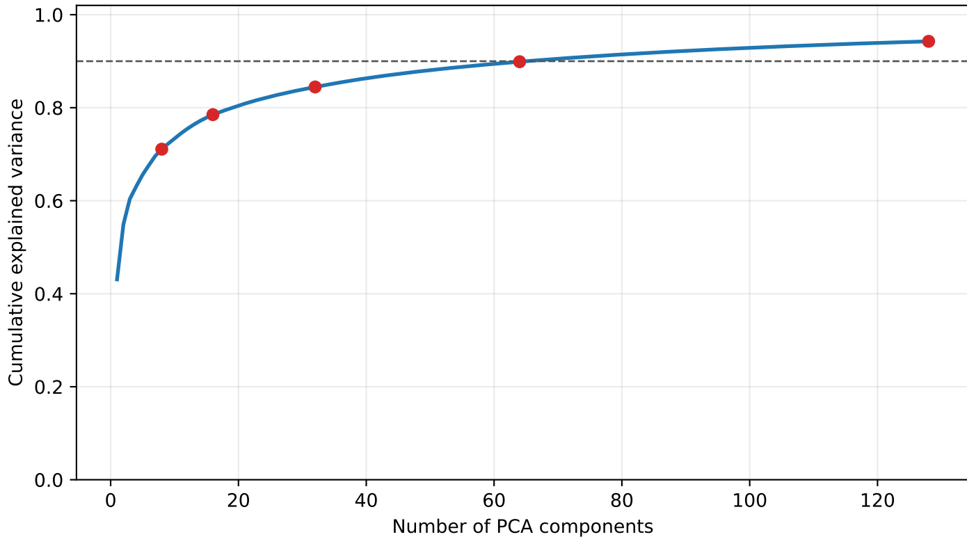
K-L/PCA Cumulative Explained Variance
