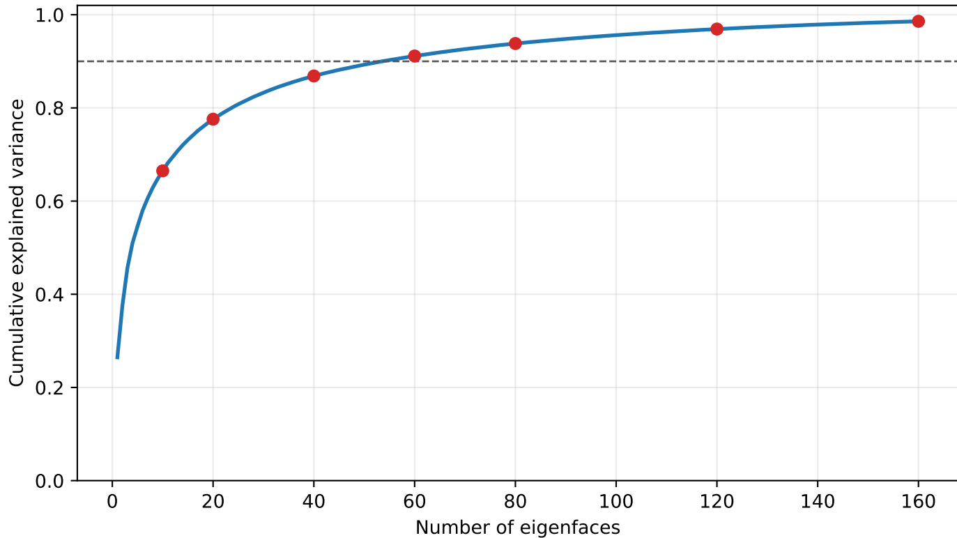
Eigenfaces Cumulative Explained Variance
