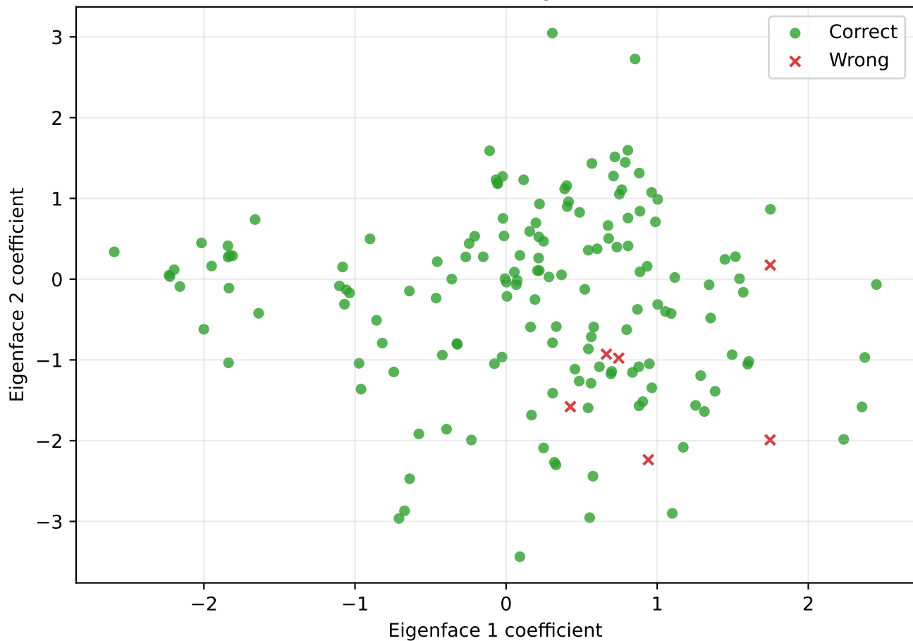
Test Faces in the First Two Eigenface Dimensions
