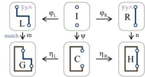
Fig. 7. A double-pushout production rule. The left side L is matched with G . L is cut from G and R is glued in its place to make H .
