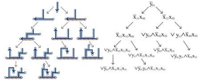
Fig. 12. A decision tree of possible gluing operations starting with \overline{y_{01}} .
