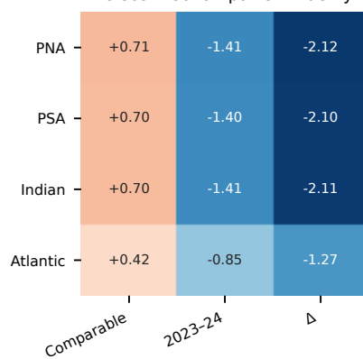
Teleconnection-pattern fidelity
