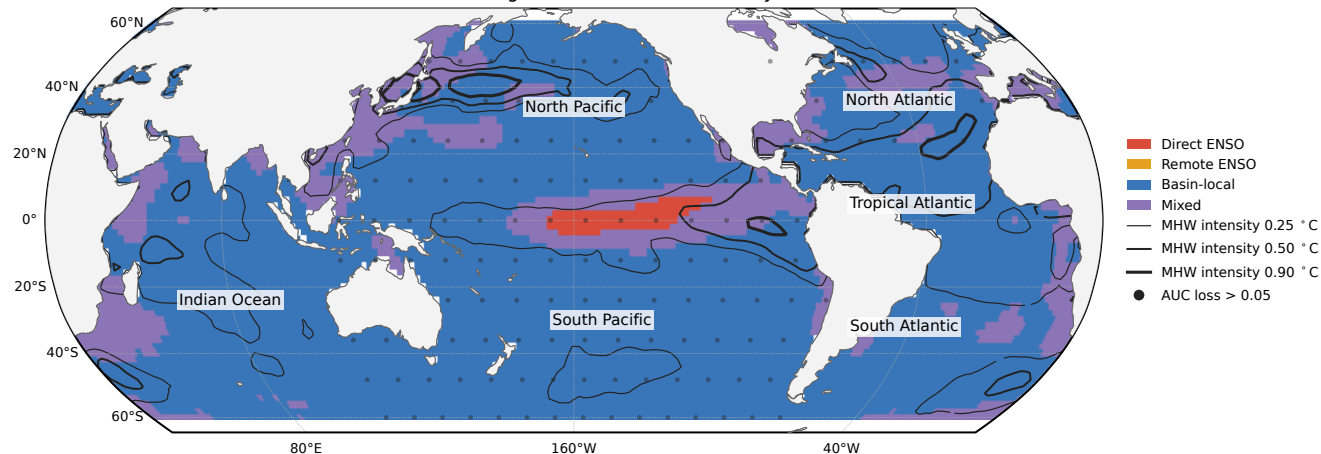
MHW driver regimes and 2023/24 intensity
