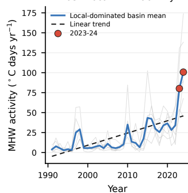
Basin-local MHW activity
