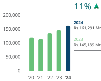
Equity Rs.Mn
