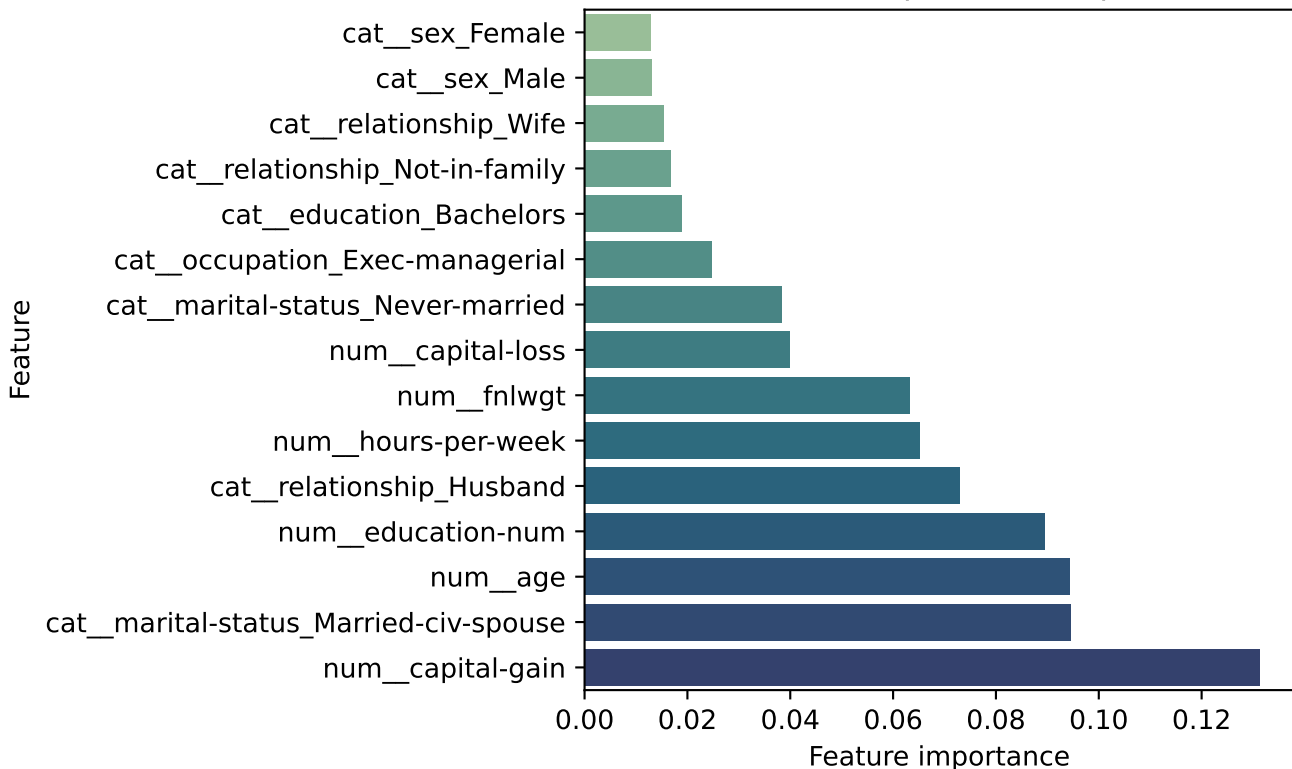
Random Forest top feature importances
