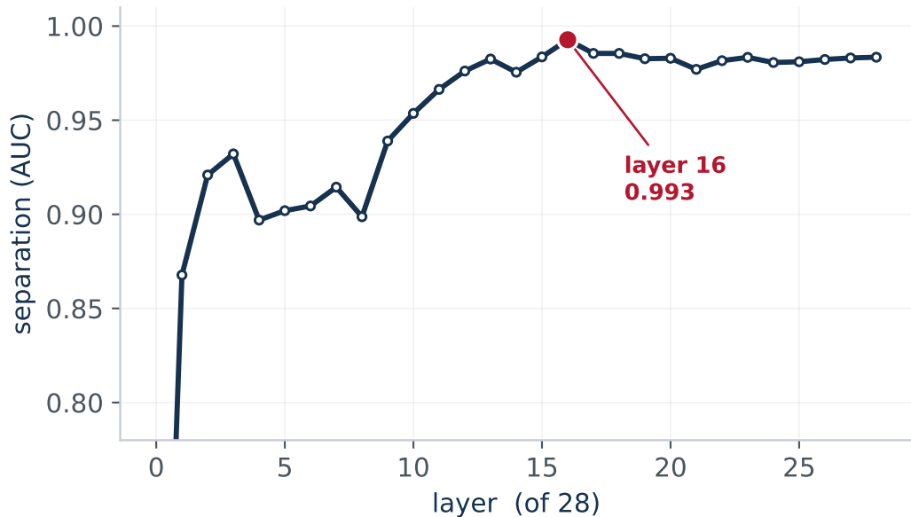
Intent is legible from the early layers on
