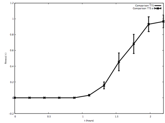
Figure 13: Performance of our algorithm on the Bazzan test averaged over 100 trials.
