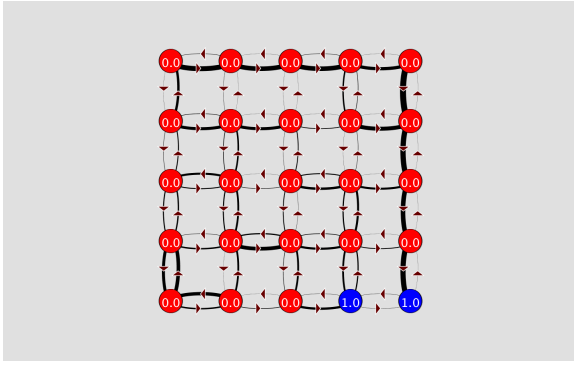
Figure 8: 5 \times 5 safety test for case 1.
