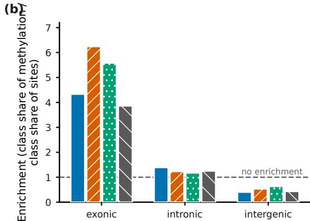
(a) absolute rate per compartment, log scale. (b) enrichment relative to each class's share of covered sites. The profiles coincide; the levels differ roughly thirty to forty fold.
