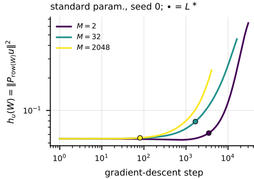
Figure 5: Trajectories of h_u(W) = \|P_{\text{row}(W)}u\|^2 under standard parameterization for M \in \{2, 32, 2048\} , seed 0; the marker is the L^* crossing.
