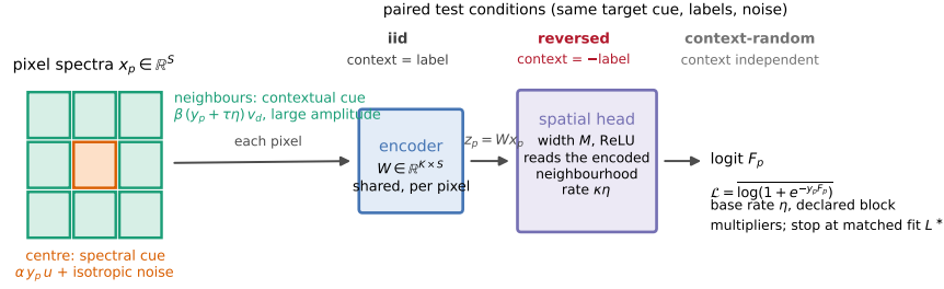
Figure 1: The serial model and the two cues. Each pixel’s spectrum passes through the shared encoder; the spatial model reads the encoded neighbourhood (a 5 \times 5 receptive field in Experiment 2; one nine-spectrum patch in Experiment 3). The contextual cue lies in the eight neighbours along large-amplitude directions that a random encoder passes; the spectral cue lies in the pixel’s own spectrum along a small-amplitude direction that, in the low-accessibility settings, requires encoder alignment. Evaluation under iid, reversed and context-random contexts measures reliance and failure.
