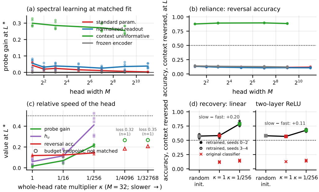
Figure 3: Experiment 2 at matched fit L^* = 0.30 (points are seeds, lines means). (a) Spectral probe gain against head width by arm. (b) Accuracy under context reversal. (c) Whole-head rate multiplier \kappa at M = 32 : probe gain, h_u and reversal accuracy; open markers are single-seed budget endpoints (losses shown). (d) Recovery: reversal accuracy of a fresh entire head ( M = 32 ) retrained for 20,000 steps on context-random images from frozen L^* encoders (random initialization, \kappa = 1 , \kappa = 1/256 ; paired initialization and common data within seed), original classifiers as crosses; linear encoder (added seeds open) and two-layer ReLU encoder; squares are means.
