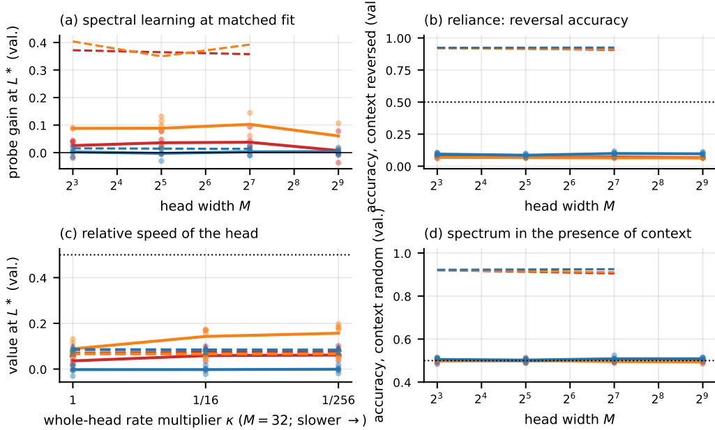
Figure 4: Experiment 3 at L^* = 0.30 , validation patients, three seeds. (a) Probe gain against width (high accessibility blue; low accessibility \gamma = 30 red, \gamma = 10 orange; comparator dashed). (b) Reversal accuracy. (c) Rate multiplier at M = 32 : probe gain (solid), reversal (dashed). (d) Accuracy with uninformative context.
