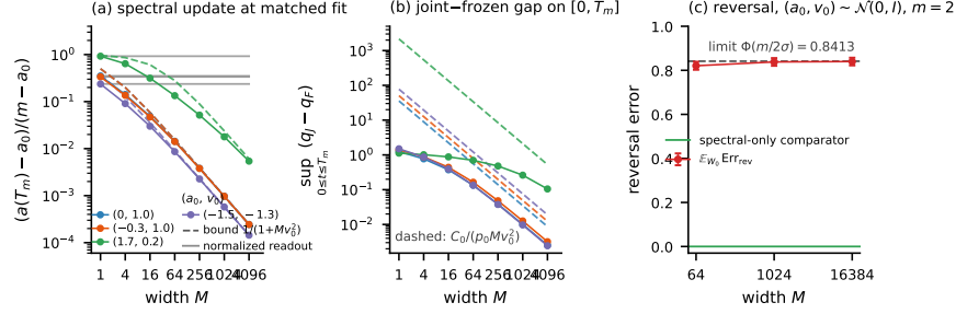
Figure 2: The exact mechanism (Theorem 1; m = 2.9 unless stated). (a) Spectral update fraction u_M/\Delta at the matched margin against width M for four initializations (a_0, v_0) (solid), the bound 1/(1 + Mv_0^2) (dashed) and the normalized readout of part (c) (grey, flat at the M = 1 value). (b) Joint-minus-frozen margin gap with the bound C_0/(p_0 M v_0^2) (dashed). (c) Expected reversal error over (a_0, v_0) \sim \mathcal{N}(0, I_2) against M for m = 2 with the limit \Phi(m/2) ; the spectral-only comparator has error zero.
