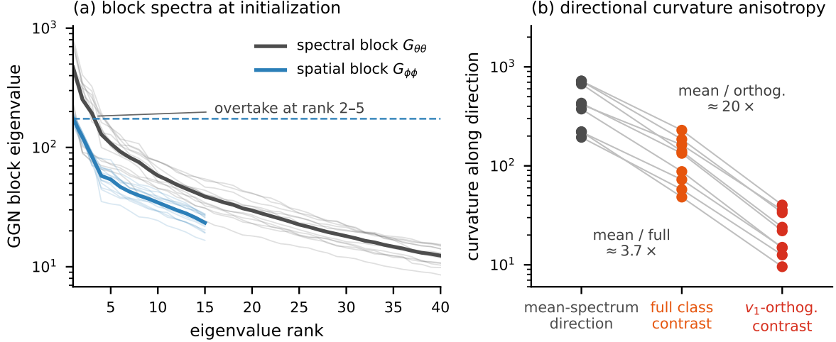
Figure 1: Directional curvature anisotropy at initialization (breast QCL, M=192 , 3 seeds \times 4 batches). (a) GGN block eigenvalue spectra: thin lines are individual measurements, thick lines their means; the dashed line marks the spatial block’s top eigenvalue, which overtakes the spectral spectrum at rank 2–5. (b) Spectral curvature along three input directions, for each of the nine measurements whose batch contains both classes (3 seeds \times 3 batches at M=192 ); thin grey lines join the three values of one measurement. Left: the leading input direction v_1 , i.e. the mean-spectrum direction. Middle: the full, un-orthogonalized CancerEpi–CAS class contrast, which retains its v_1 component ( |\cos(d, v_1)| = 0.45 ). Right: that same contrast after orthogonalization against v_1 . Curvature is 3.7\times lower along the full contrast than along v_1 (range 2.6\text{--}4.8\times ) and 20\times lower along the v_1 -orthogonalized contrast (range 12\text{--}28\times ): the large anisotropy is a statement about the v_1 -orthogonal part of the contrast, not about the class contrast as a whole.
