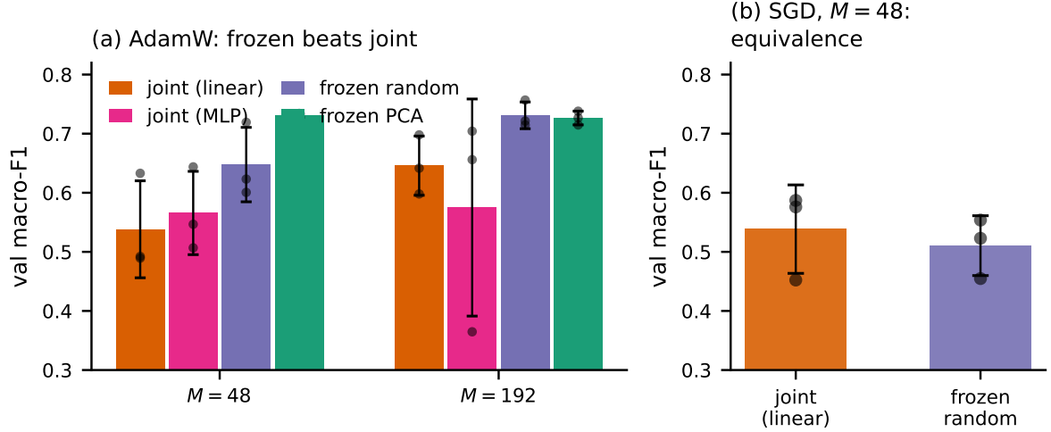
Figure 2: Controlled retraining study, original protocol (breast QCL fold 0; bars: mean over 3 seeds, whiskers: sd, dots: individual seeds). (a) Under AdamW, on the pre-registered final-window metric, every frozen arm scores higher than every joint arm at both widths; the ordering reverses under a best-validation policy (Table 4). Both orderings are confounded by the clip-scope and batch-normalization-affine asymmetries described in the text and do not survive the matched protocol (Table 5). (b) Under momentum SGD — an optimizer-family control, not an instantiation of Theorem 27’s gradient flow — joint training and frozen-random show no resolvable best-validation difference at n = 3 , while their final-window gaps differ in sign between the two widths.
