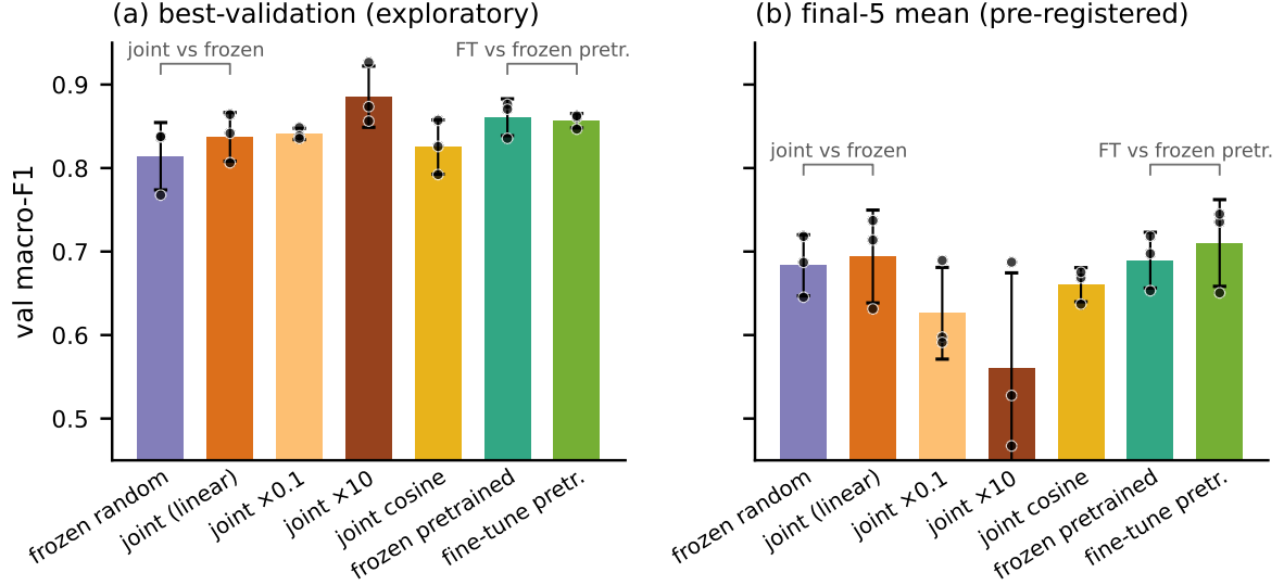
Figure 3: Controlled study, matched protocol : identical batch-normalization affine treatment, \phi -only clipping and saved best-validation checkpoints in every arm ( M=48 , AdamW, 3 seeds; dots are seeds, bars are seed means, whiskers sd). (a) Best-validation macro-F1 — a post-hoc maximum over 60 evaluations on the same 28-core fold-0 validation split, hence exploratory and selection-optimistic. (b) The pre-registered metric, the mean over the final 5 epochs. Brackets mark the two pre-registered pairs; no pre-registered difference is resolvable at n = 3 under either policy.
