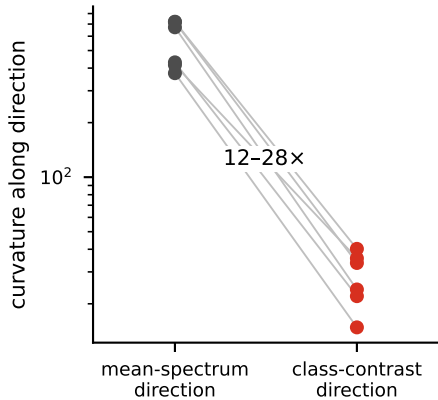
(b) direction-wise starvation
