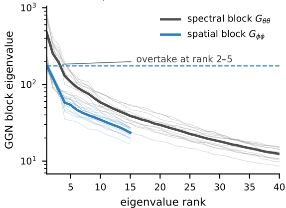
(a) block spectra at initialization
