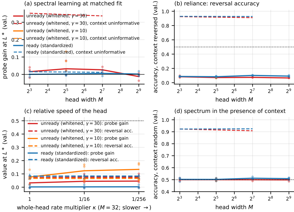
Figure 4: Experiment 3 at L^* = 0.30 on validation patients (three seeds; points are seeds). (a) Spectral probe gain against width in the two regimes, with the uninformative-context comparator dashed. (b) Accuracy under context reversal. (c) Whole-head rate multiplier at M = 32 . (d) Accuracy with an uninformative context: what the model does from the spectrum in the presence of context.
