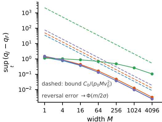
(b) joint–frozen margin gap
