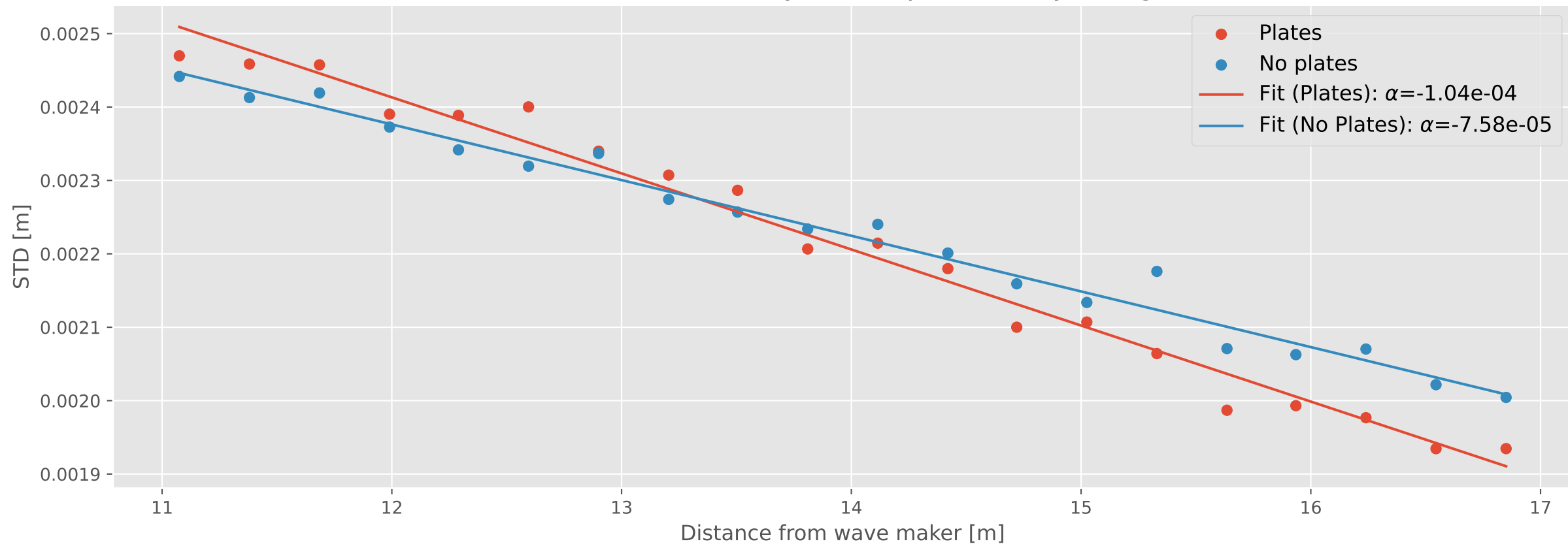
Standard deviation of synthetic probe array along tank
