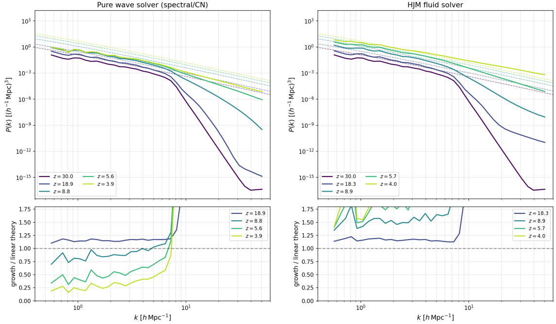
Figure 1. Growth validation on a 15 h^{-1}\text{Mpc} , 256^3 grid with m_a = 10^{-23} \text{ eV} . Solid curves: measured |\psi|^2 power spectra; dashed: linear theory; bottom panels: measured growth relative to the z = 30 snapshot divided by the linear-theory growth. Left: pure wave solver — growth follows linear theory until the velocity-Nyquist limit ( z \simeq 9 here, section 4.3) and freezes beyond it. Right: HJM fluid solver on the same configuration — growth continues through z = 4 ; the high- k excess at late times is nonlinear growth.
