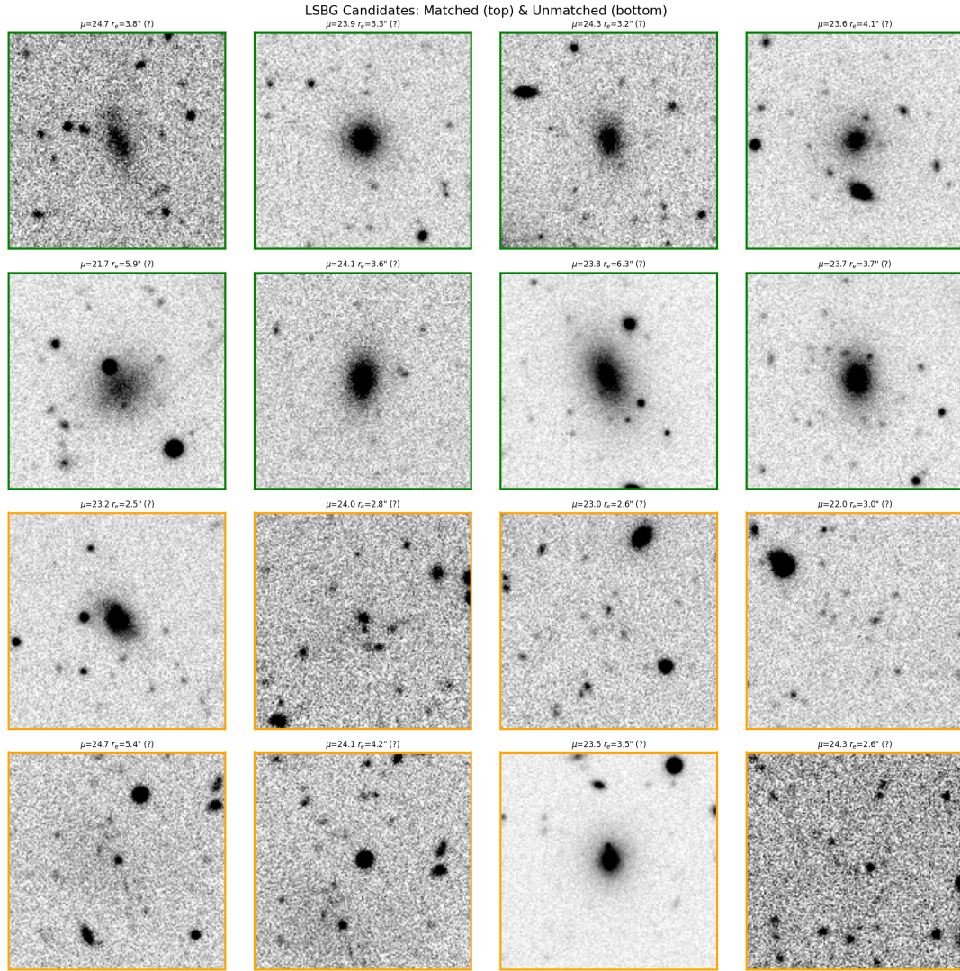
Figure 10.5: LSBG candidate cutouts ( 42'' \times 42'' ). Top two rows: sources matched with Du+2024 reference (green). Bottom two rows: additional OGFinder detections not in reference (orange). Labels show catalog number, \mu_{\text{eff}} , r_e , and grade.
