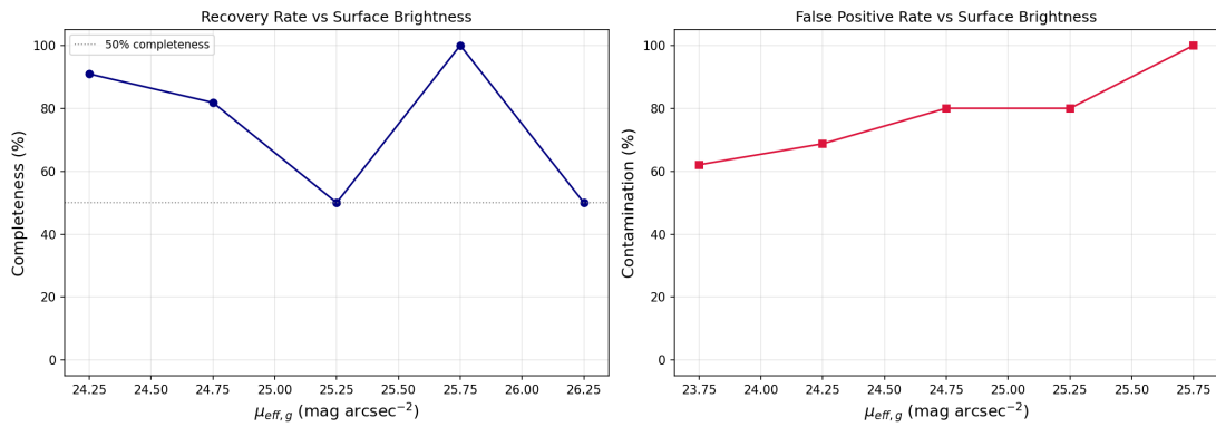
Figure 10.4: Left: completeness (recovery rate) vs. \mu_{\text{eff}} . Right: contamination (false positive rate). Du+2024 uses XGBoost ML filtering; OGFinder uses Sérsic-based grading.
