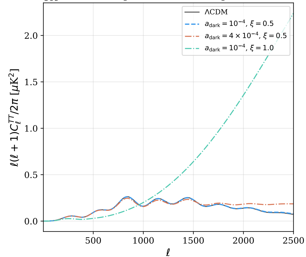
1e9 CMB Temperature Power Spectrum
