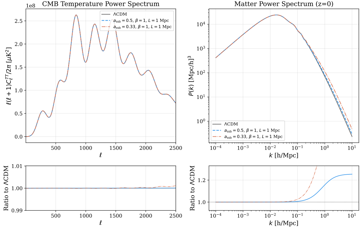
Figure 15: Symmetron: P(k) enhancement confined to k \gtrsim 1/L and switching on only after a_{\text{ssb}} (earlier symmetry breaking gives a stronger boost); large scales and the CMB are essentially unchanged. For a_{\text{ssb}} \geq 1 the model reduces to GR exactly.
