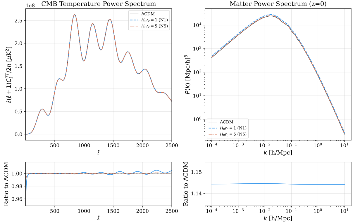
Figure 14: nDGP: scale-independent enhancement of P(k) ( \sim 14\% for N1, \sim 3\% for N5 at z = 0 , consistent with the \sim 15\% linear N1 boost of Winther et al. 2015), with the CMB essentially unchanged.
