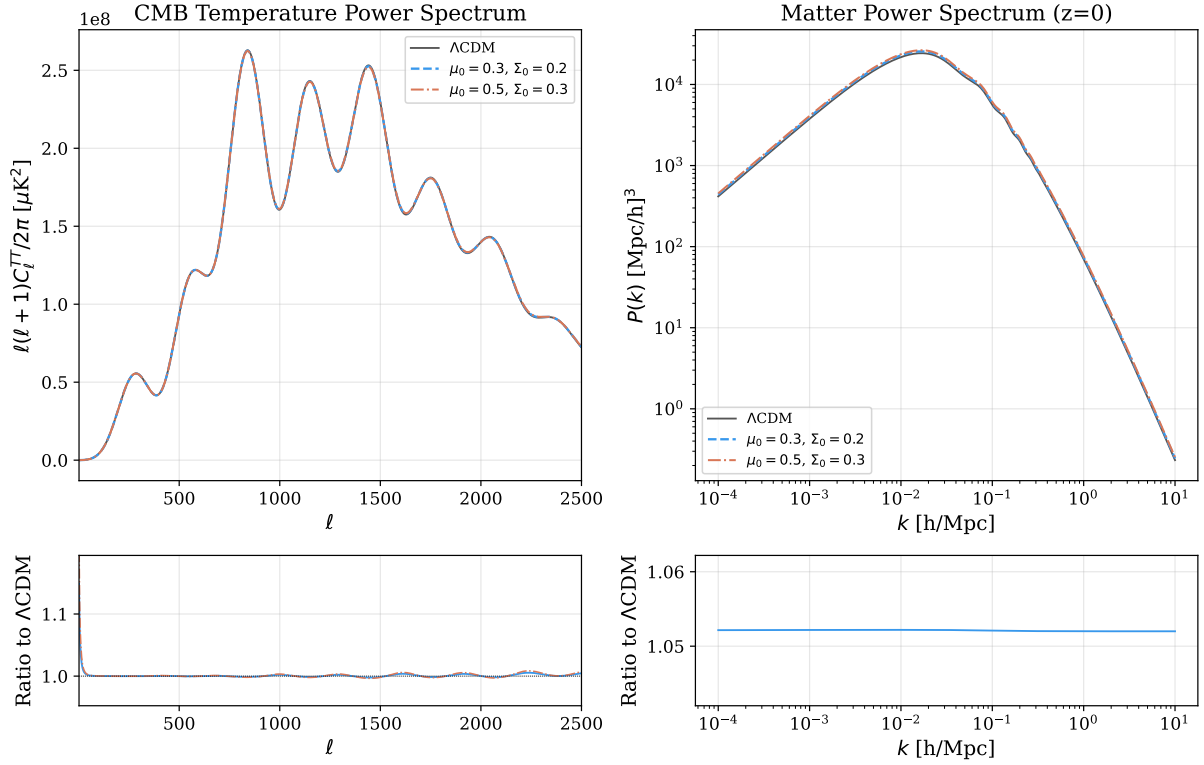
Figure 12: \mu - \Sigma MG: Modified lensing and Poisson equations affect the CMB through the ISW effect and lensing. The matter P(k) shows changes through the modified growth rate.
