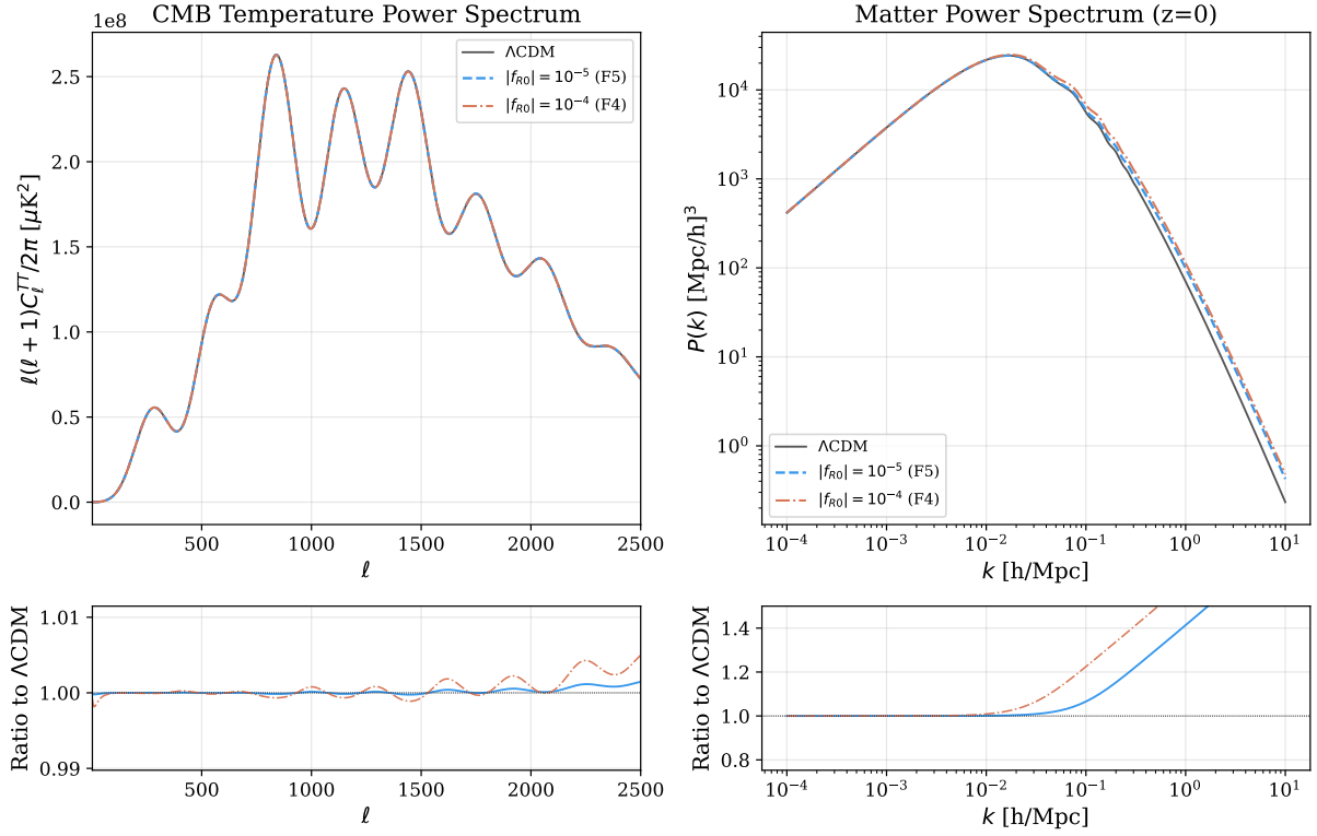
Figure 13: f(R) Hu-Sawicki: the CMB TT spectrum is essentially unchanged (sub-percent lensing differences at high \ell ), while P(k) is enhanced for k \gtrsim 0.01 h/\text{Mpc} with the characteristic scale-dependent shape, stronger for F4 than F5. Validation: linear F5 boost at k \sim 1 h/\text{Mpc} is \sim 40\% , consistent with the Winther et al. (2015) code comparison.
