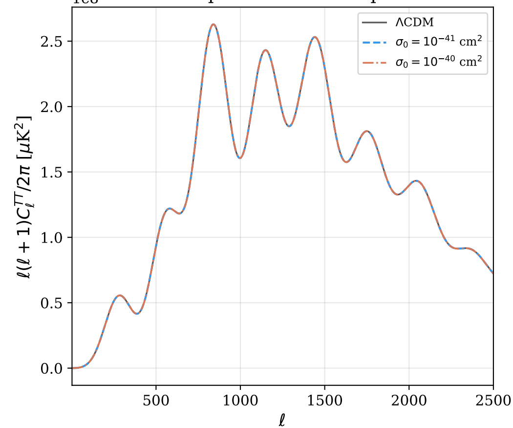
CMB Temperature Power Spectrum
