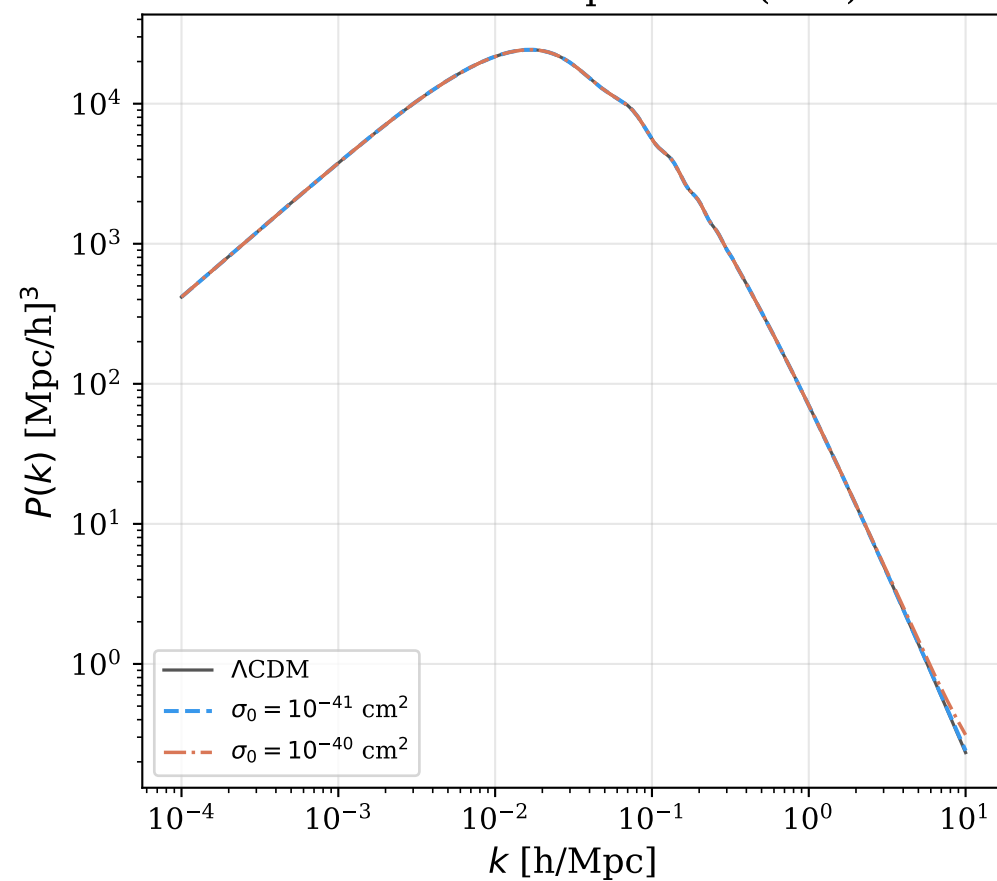
Matter Power Spectrum (z=0)
