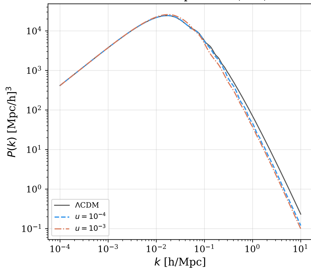
Matter Power Spectrum (z=0)
