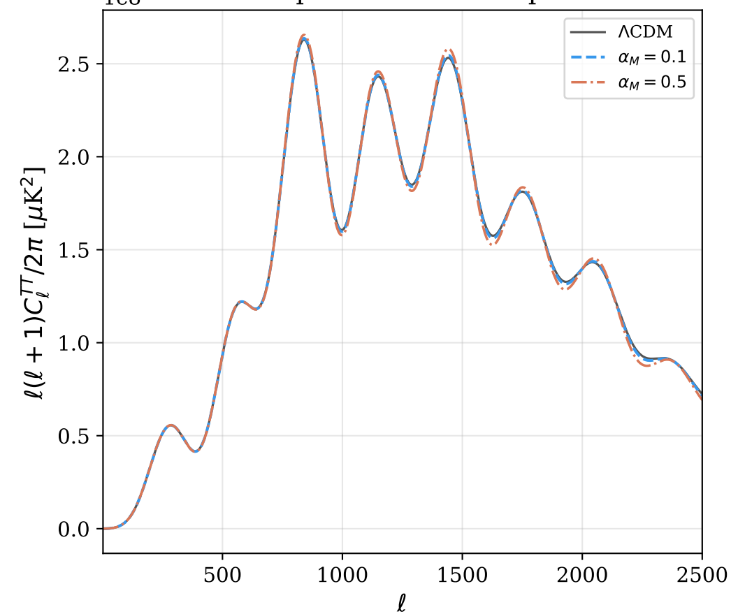
CMB Temperature Power Spectrum
