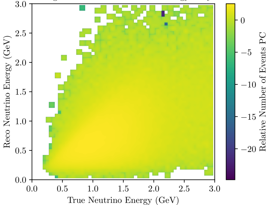
Smearing Matrix for numuCC_PC_energy_res.yaml
