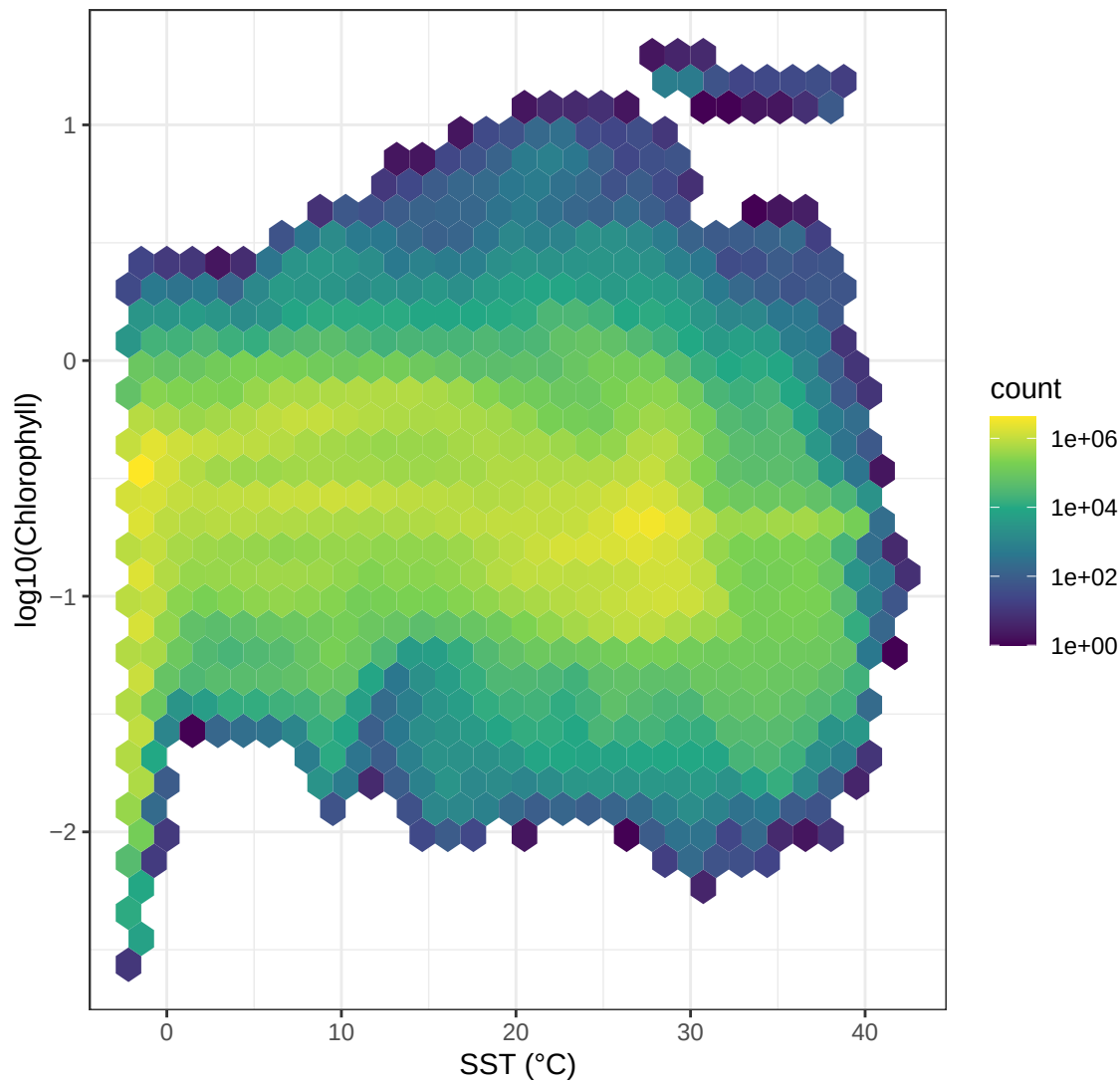
SST vs Chlorophyll Relationship (All Models and Experiments)
