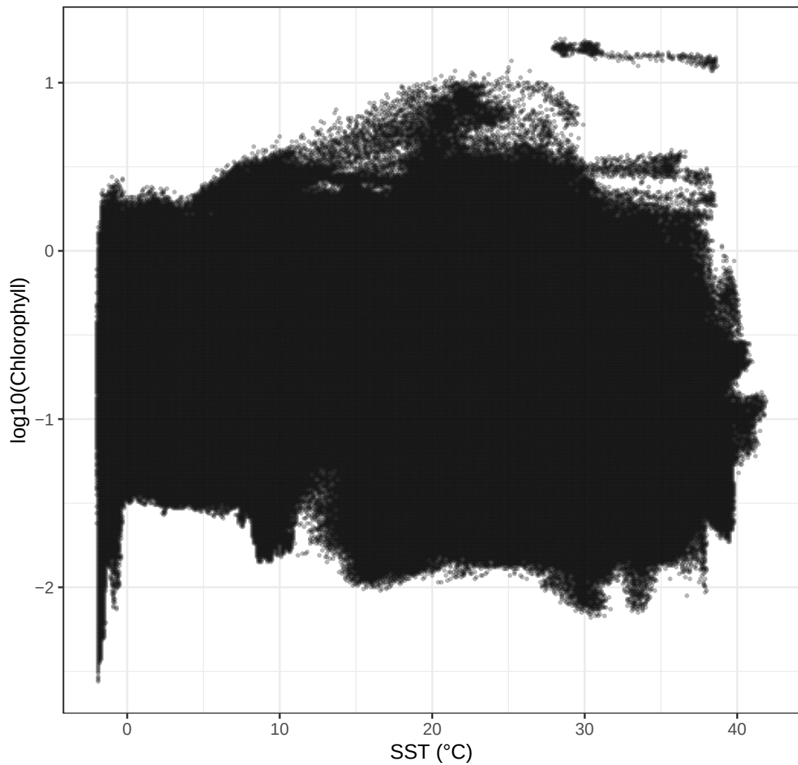
Unique SST–Chlorophyll Combinations
