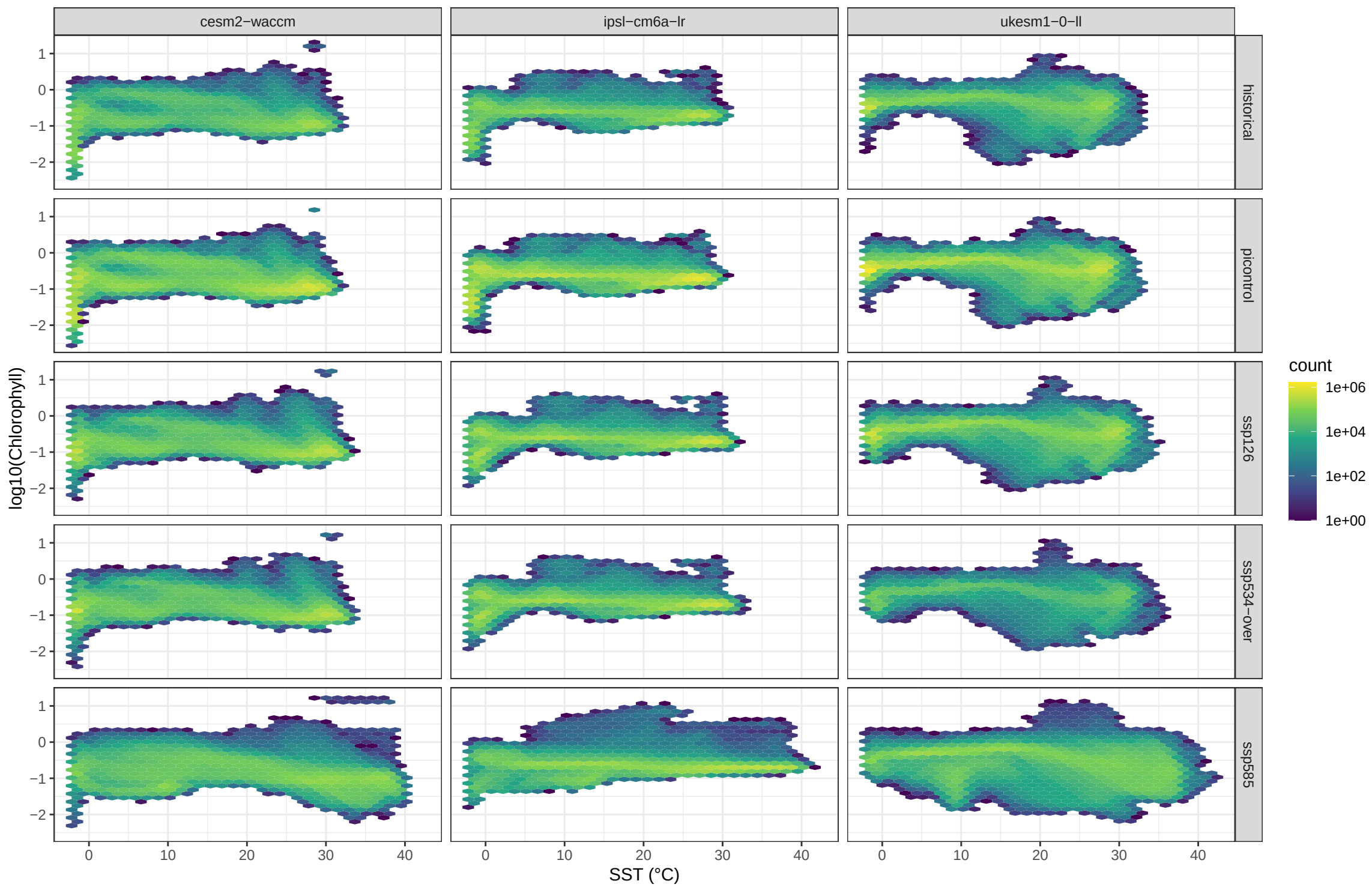
SST vs Chlorophyll by Model and Experiment
