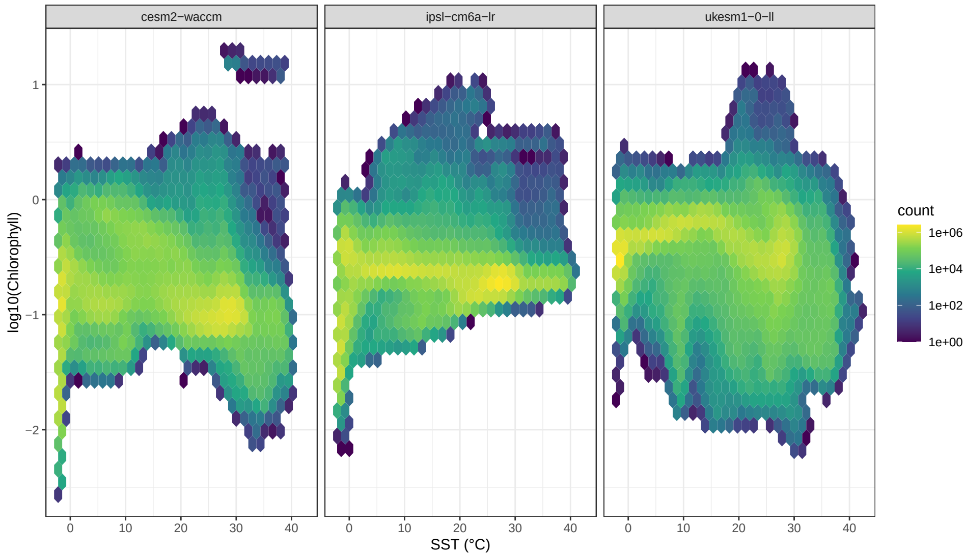
SST vs Chlorophyll Relationship by Model
