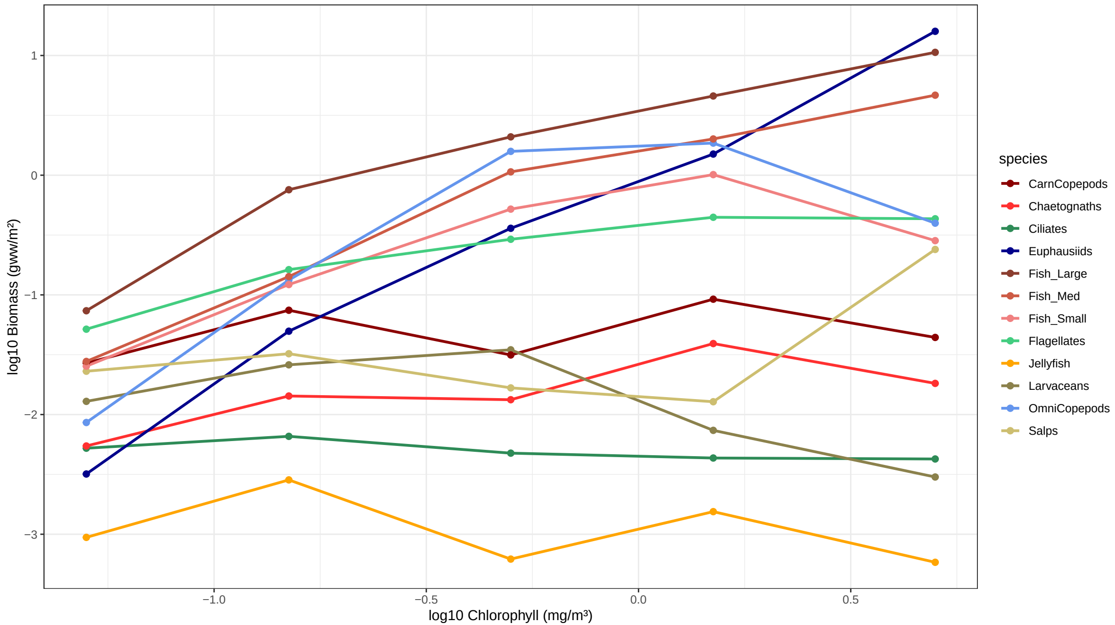
Biomass vs Chlorophyll (SST = 20°C)
