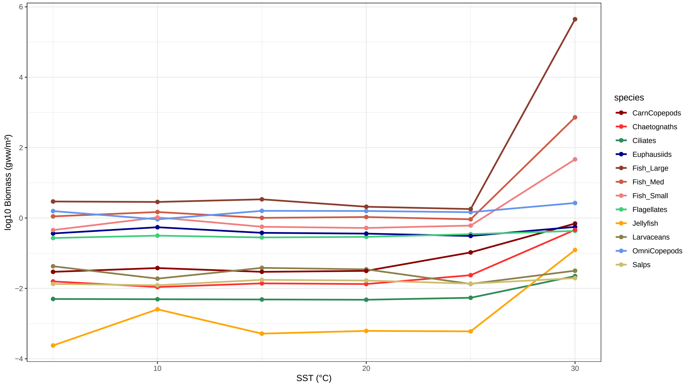
Biomass vs SST (chl = 0.5 mg/m 3 )
