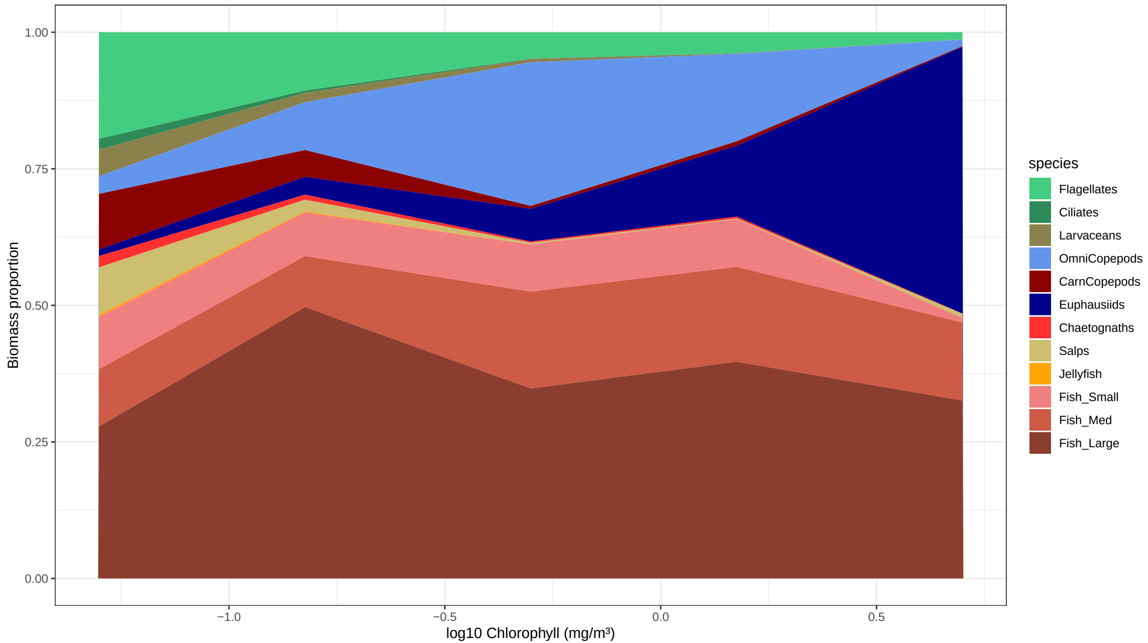
Community composition vs Chlorophyll (SST = 20°C)
