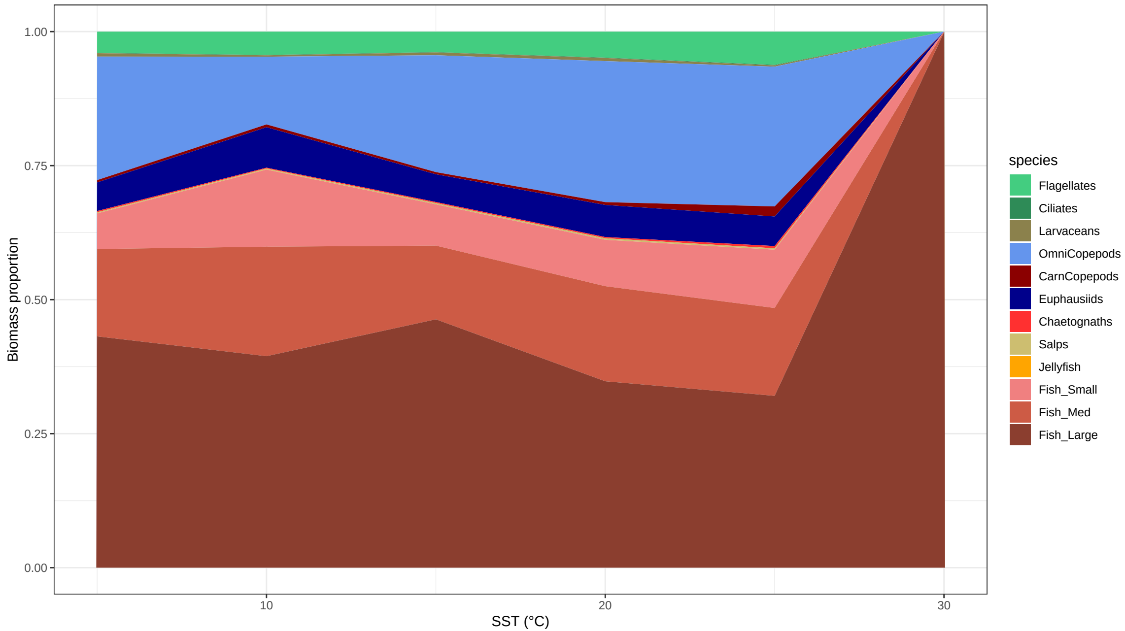
Community composition vs SST (chl = 0.5 mg/m 3 )
