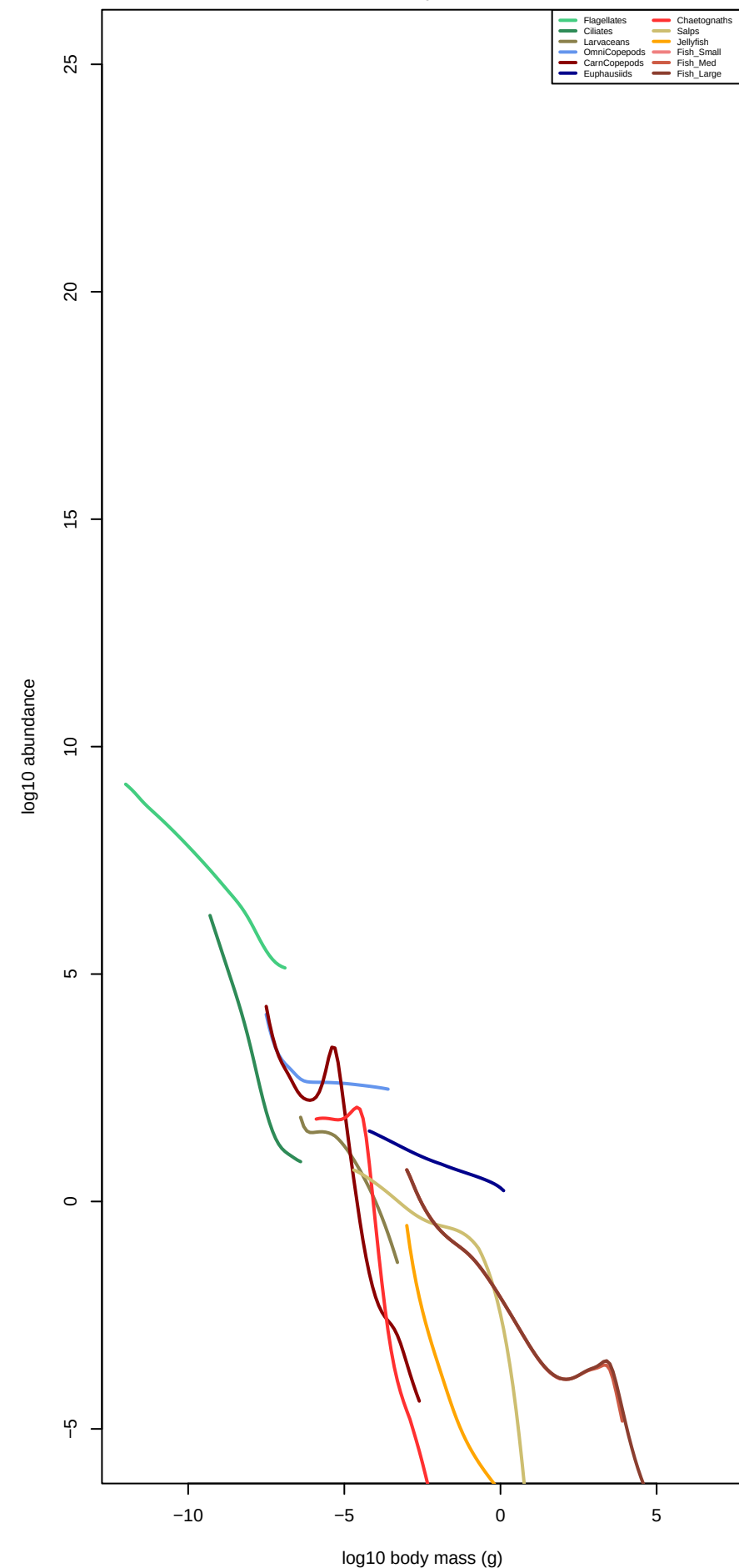
SST=20°C, chl=5.00
