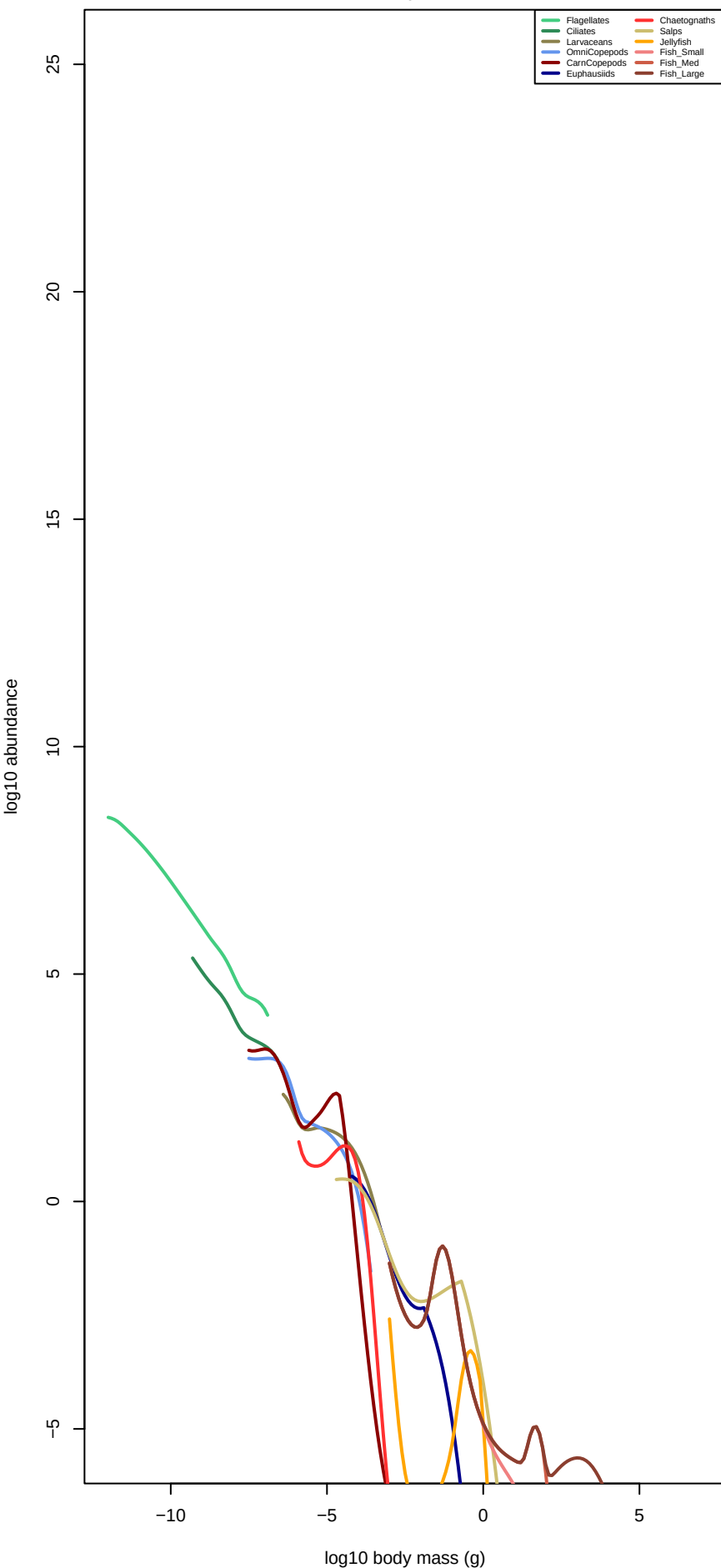
SST=20°C, chl=0.05
