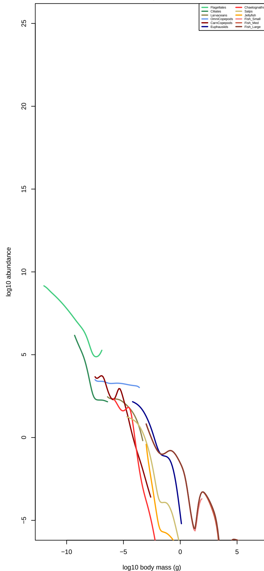
SST=20°C, chl=0.50
