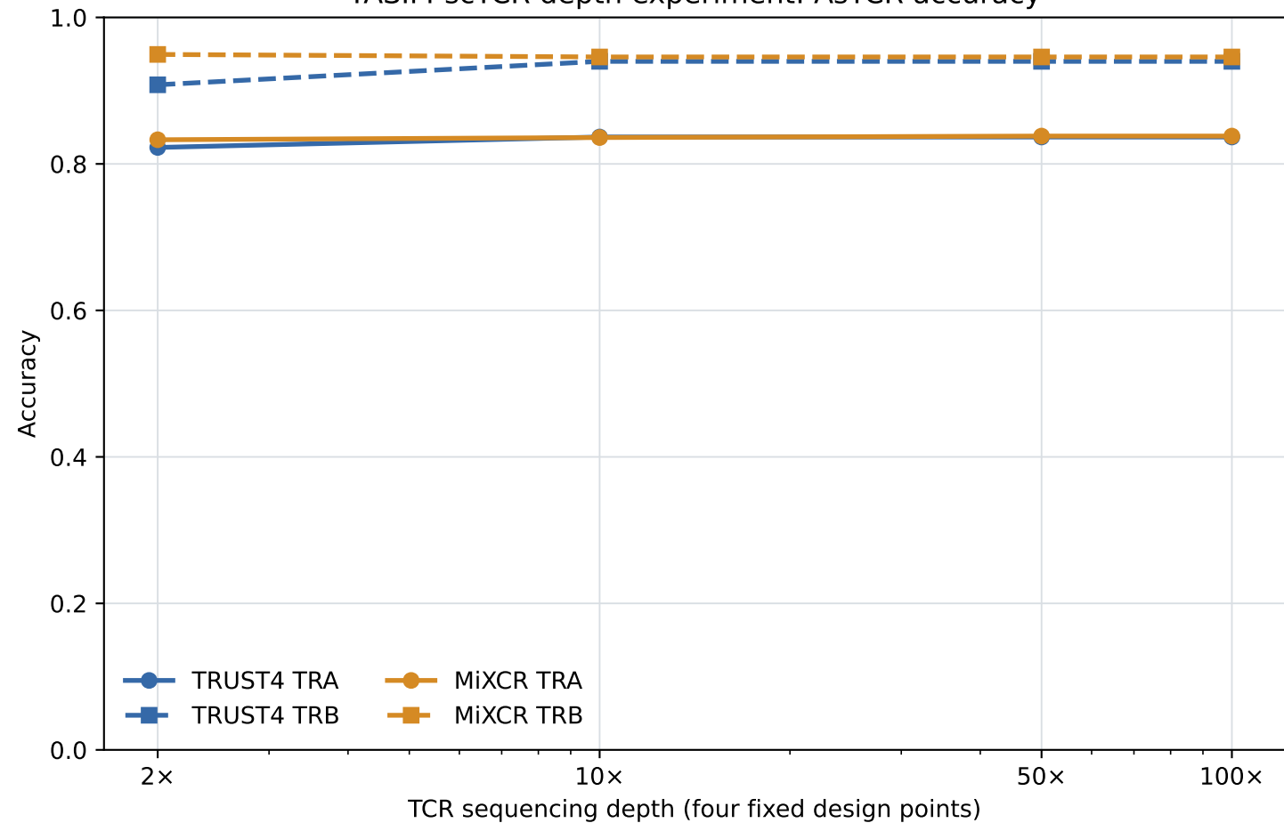
YASIM-scTCR depth experiment: AsTCR accuracy
